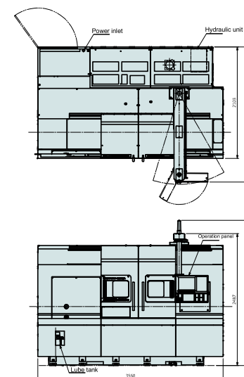
GENOS L3000-e (MYx1000)
