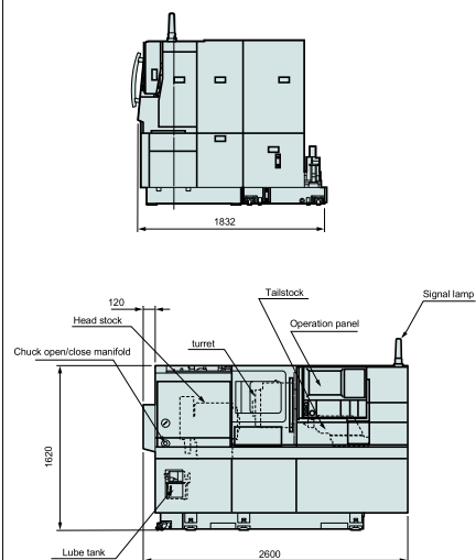
GENOS L2000-e (Lx500/Mx380) NC tailstock(Option)
